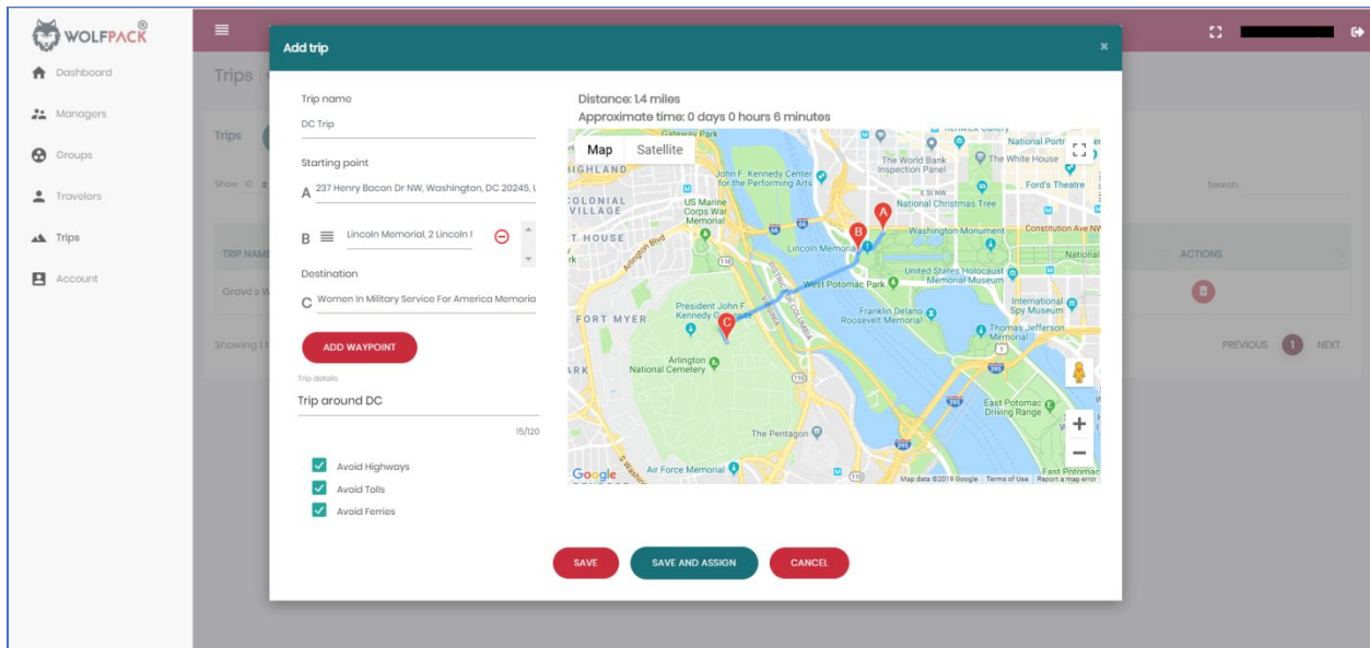
Figure 4: Trip Planning
